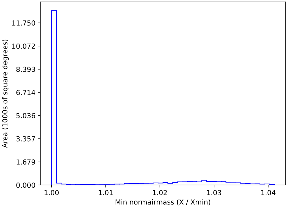
weather_cloudso1v3.4_10yrs WFD y band: Min normairmass
