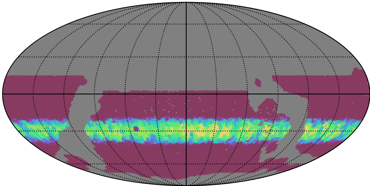
weather_cloudso1v3.4_10yrs WFD r band: Min normairmass
