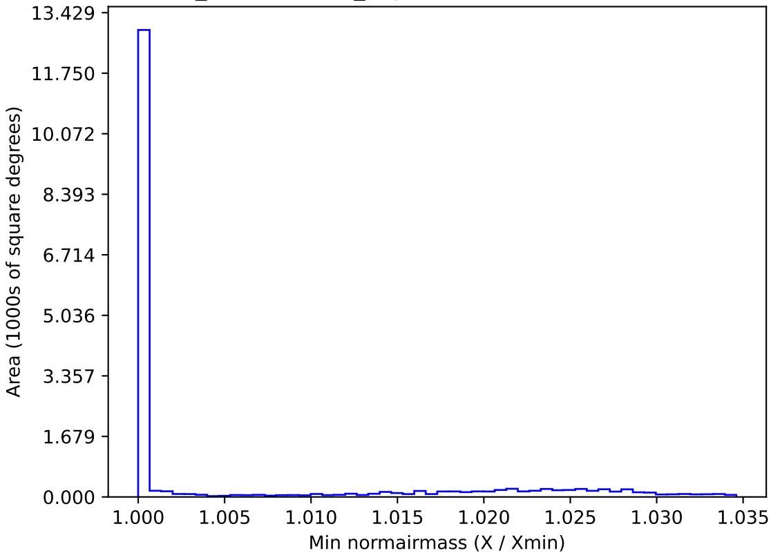
weather_cloudso1v3.4_10yrs WFD r band: Min normairmass
