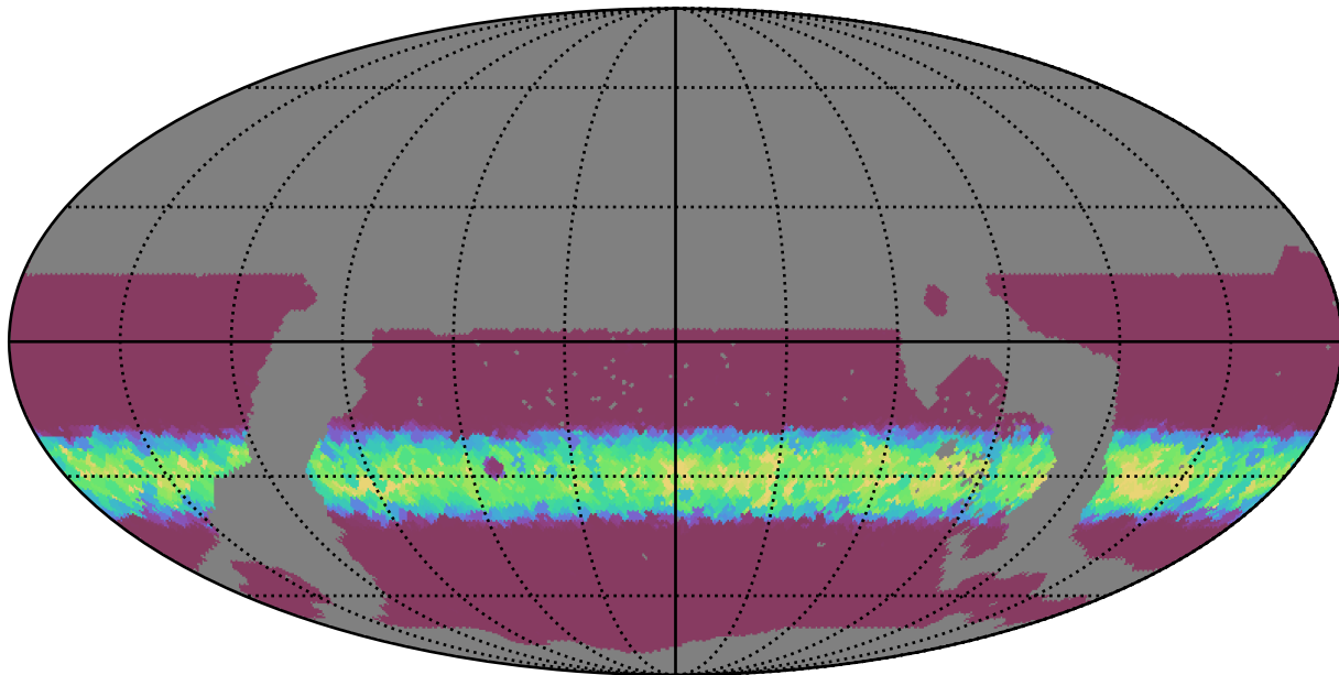
weather_cloudso1v3.4_10yrs WFD i band: Min normairmass
