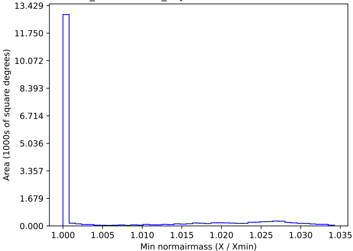
weather_cloudso1v3.4_10yrs WFD i band: Min normairmass
