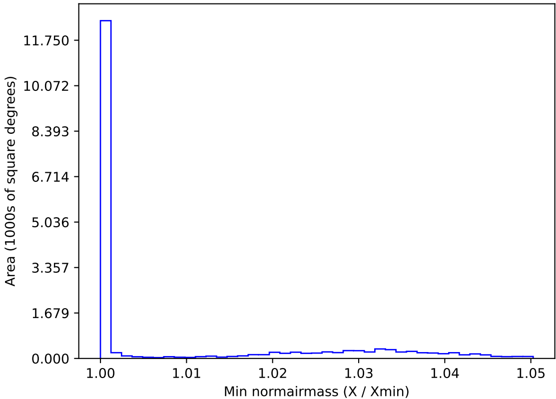
weather_cloudso1v3.4_10yrs WFD g band: Min normairmass
