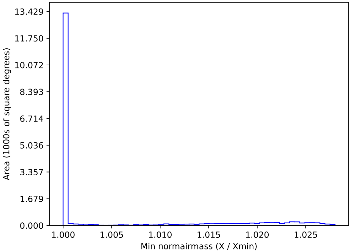
weather_cloudso1v3.4_10yrs WFD all bands: Min normairmass
