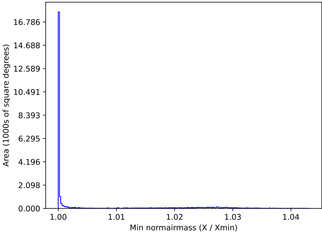
weather_cloudso1v3.4_10yrs All sky z band: Min normairmass
