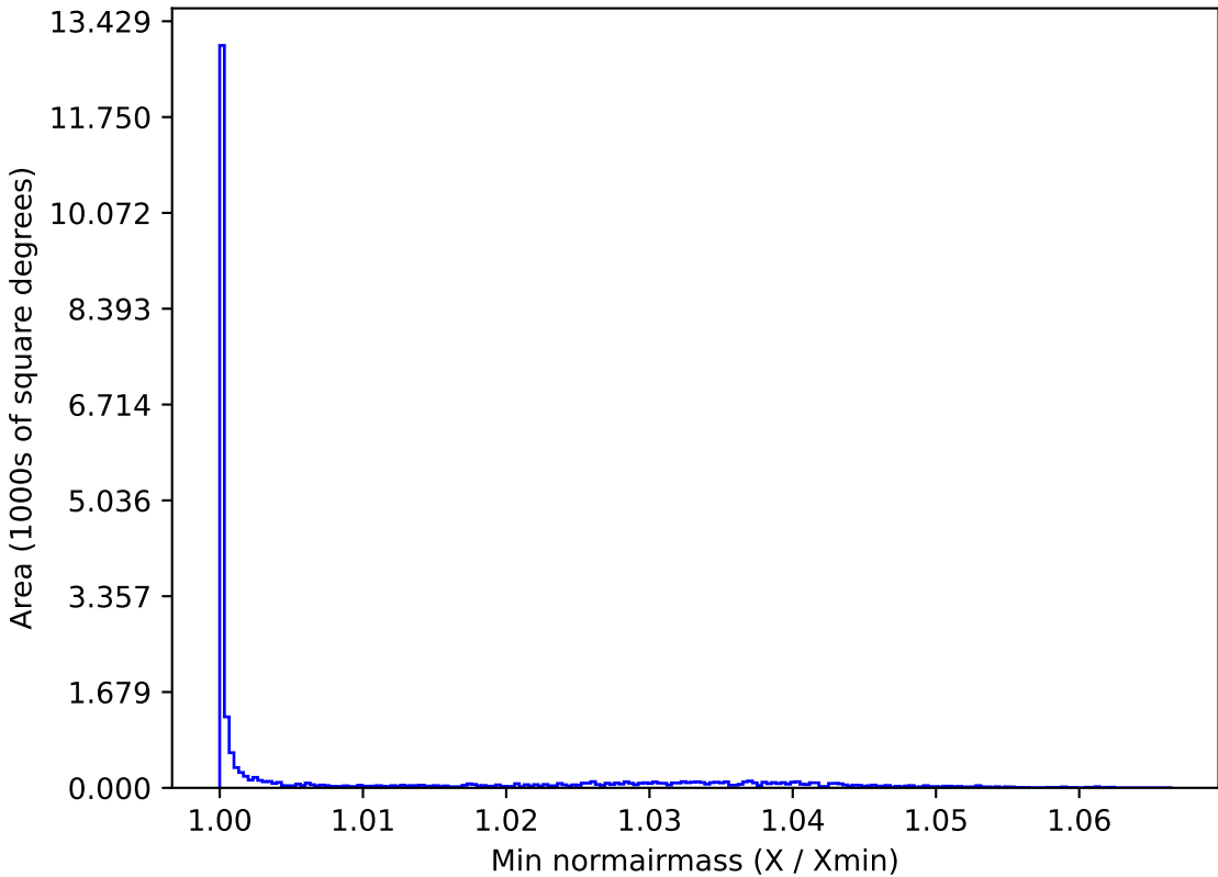
weather_cloudso1v3.4_10yrs All sky u band: Min normairmass
