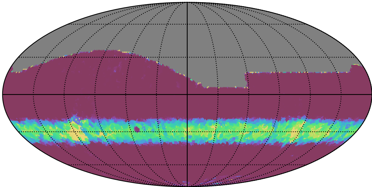
weather_cloudso1v3.4_10yrs All sky i band: Min normairmass
