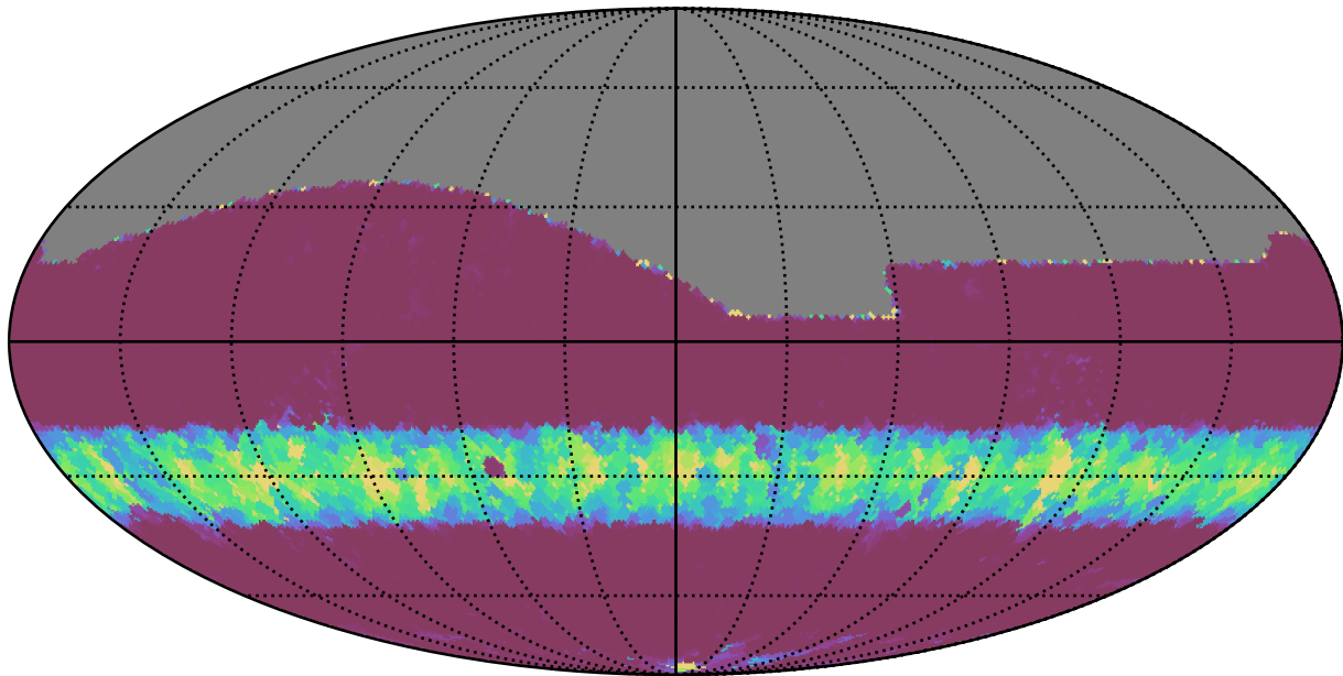
weather_cloudso1v3.4_10yrs All sky g band: Min normairmass
