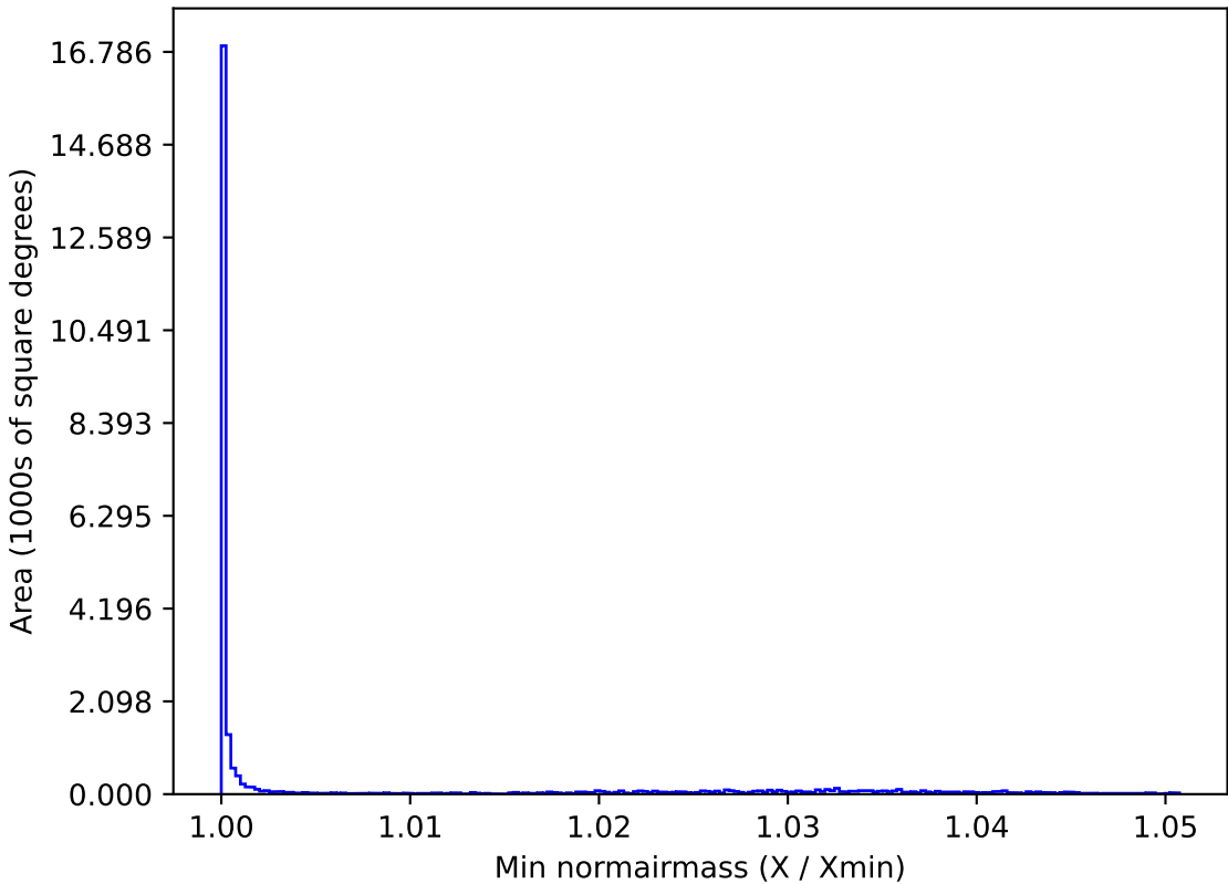
weather_cloudso1v3.4_10yrs All sky g band: Min normairmass
