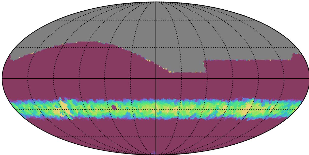
weather_cloudso1v3.4_10yrs All sky all bands: Min normairmass
