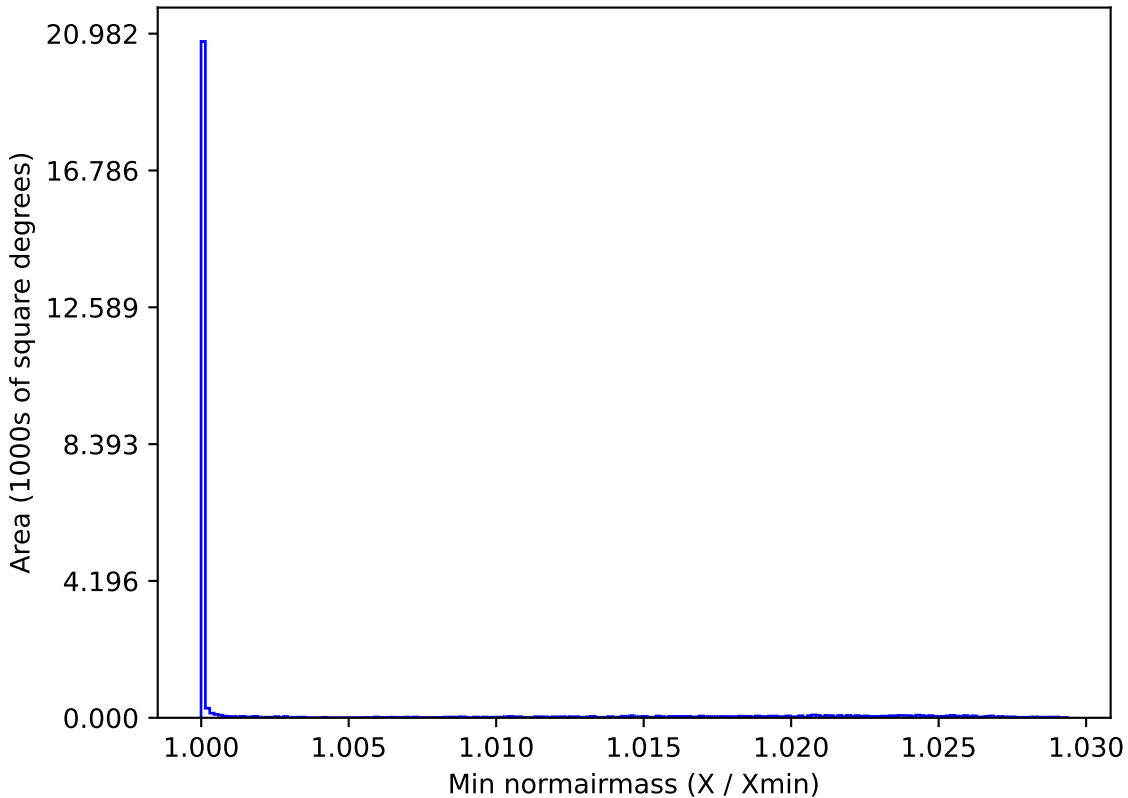
weather_cloudso1v3.4_10yrs All sky all bands: Min normairmass
