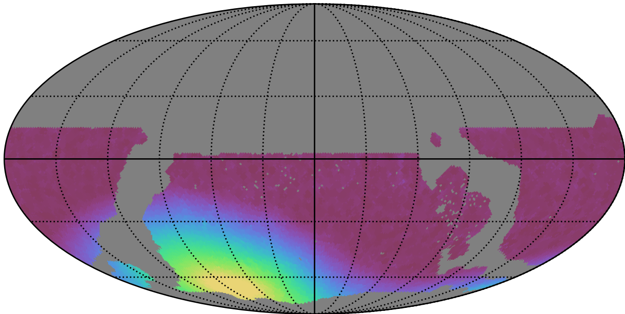
weather_cloudso1v3.4_10yrs WFD z band: Min moonDistance
