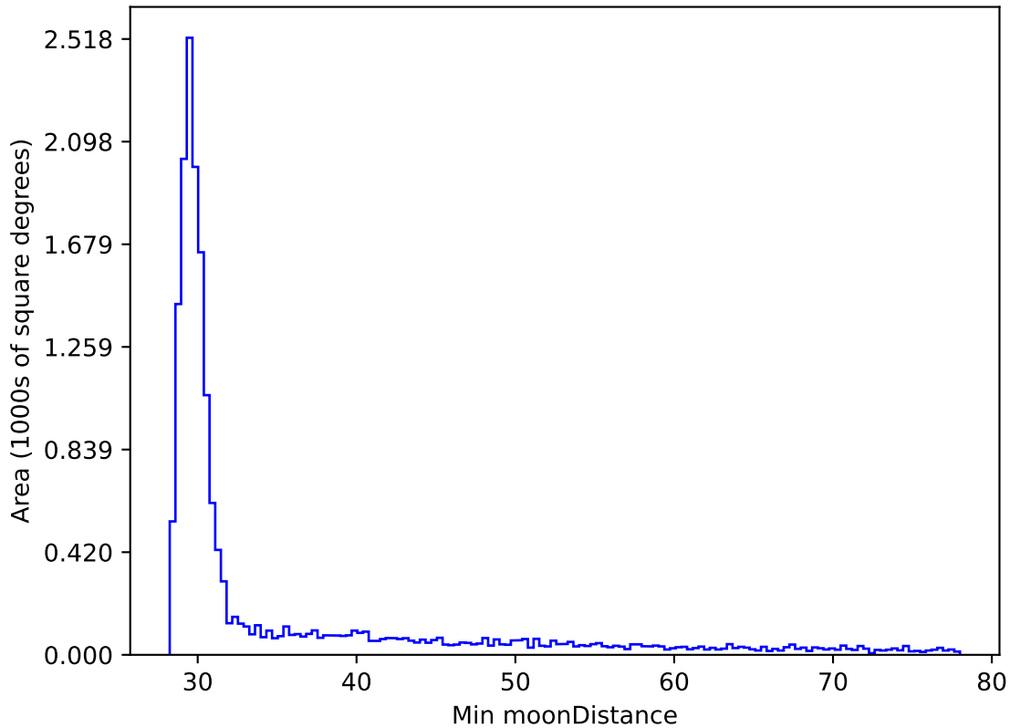
weather_cloudso1v3.4_10yrs WFD z band: Min moonDistance
