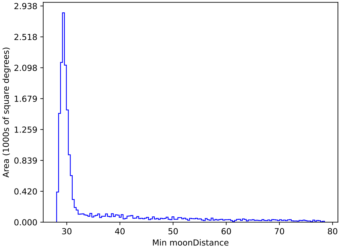
weather_cloudso1v3.4_10yrs WFD y band: Min moonDistance
