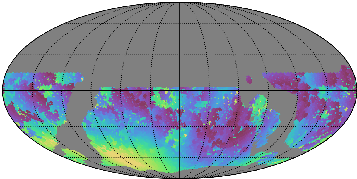
weather_cloudso1v3.4_10yrs WFD u band: Min moonDistance
