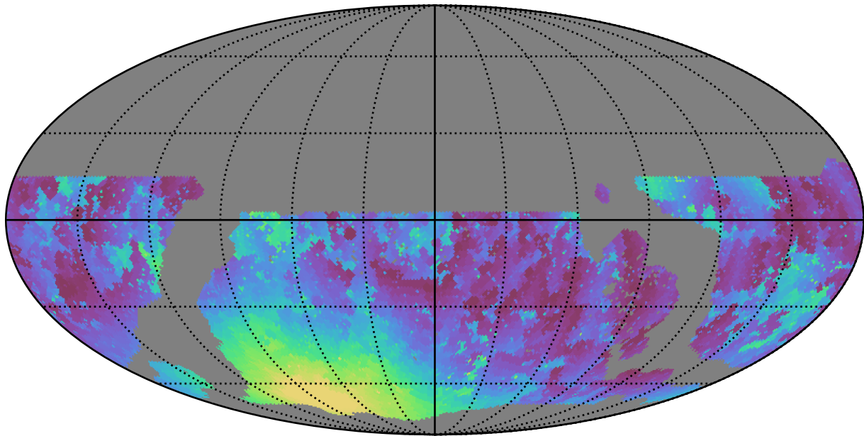
weather_cloudso1v3.4_10yrs WFD g band: Min moonDistance
