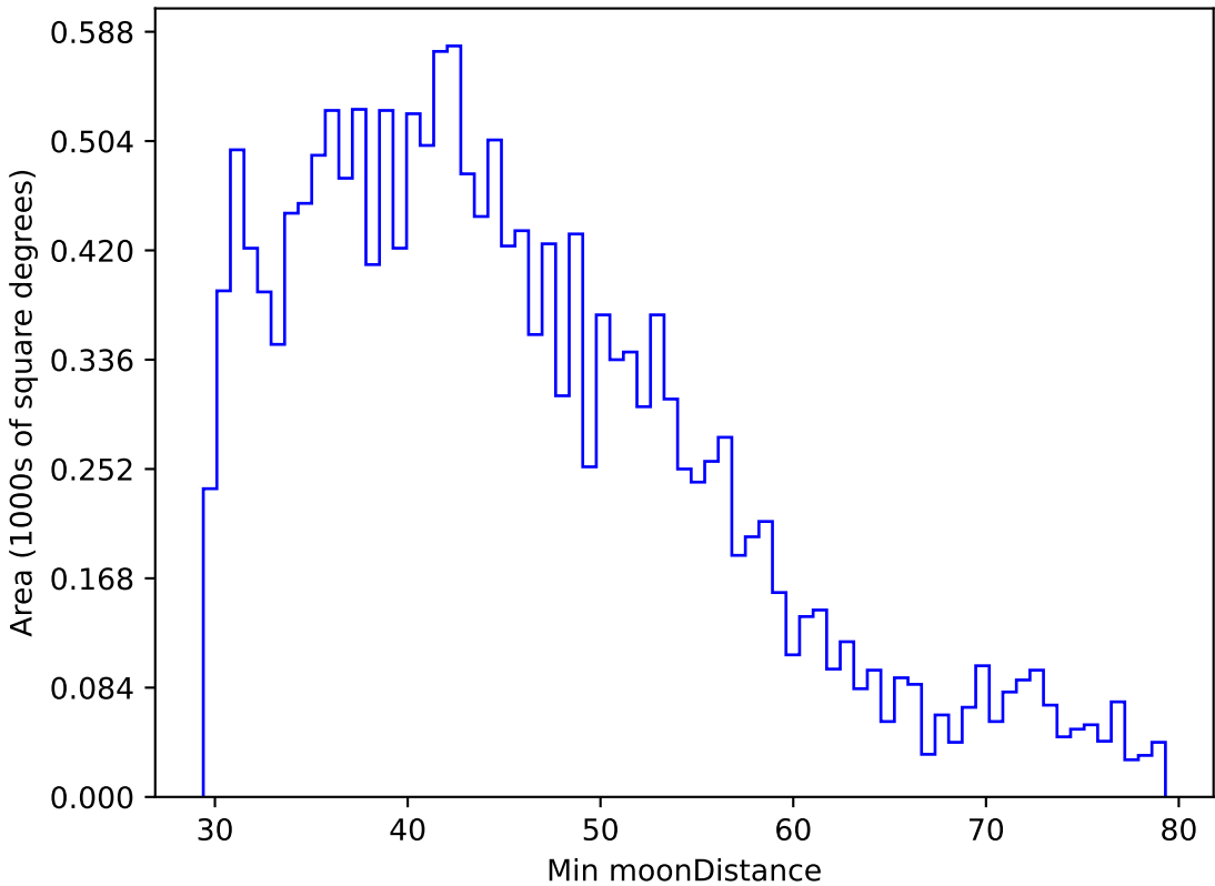
weather_cloudso1v3.4_10yrs WFD g band: Min moonDistance
