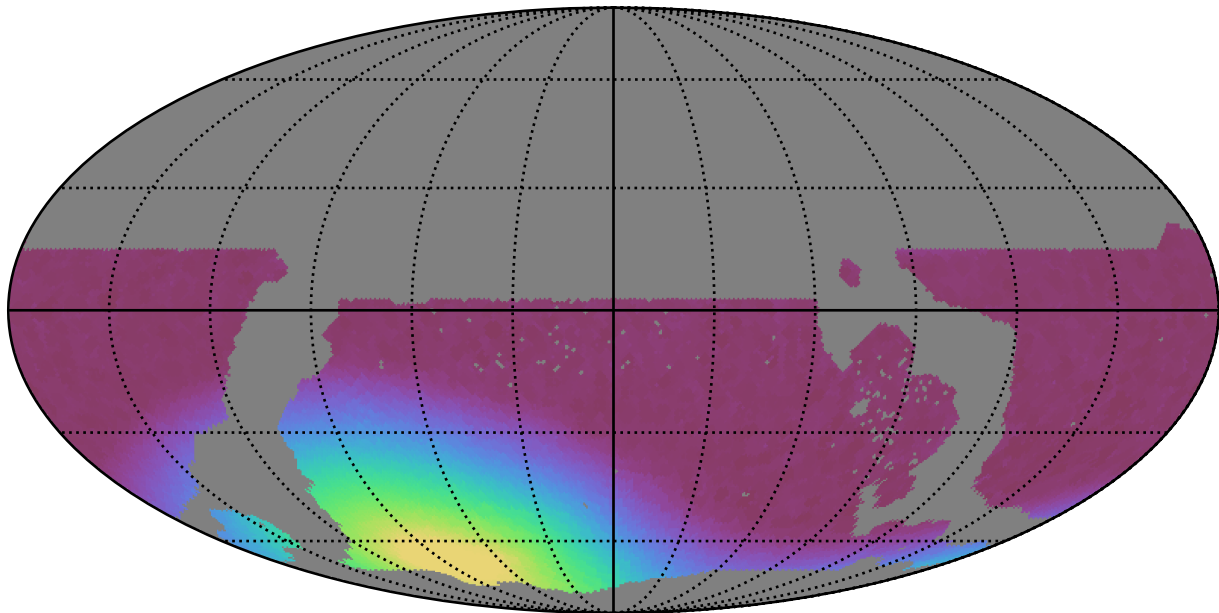
weather_cloudso1v3.4_10yrs WFD all bands: Min moonDistance
