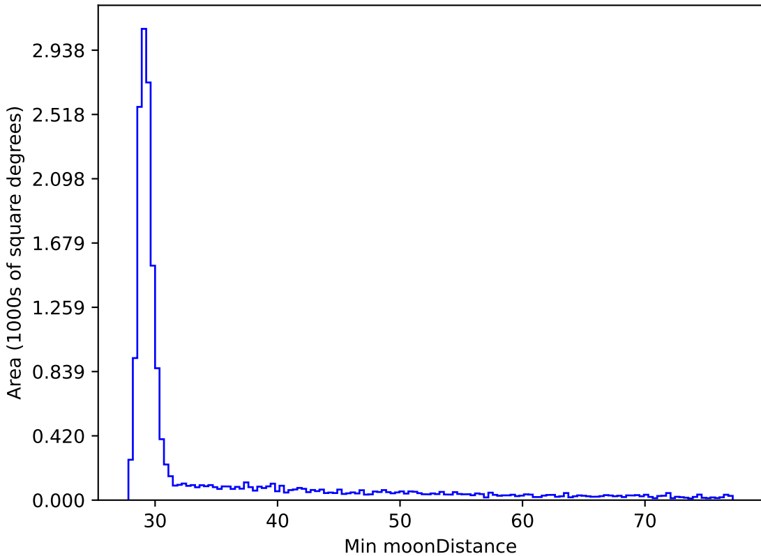
weather_cloudso1v3.4_10yrs WFD all bands: Min moonDistance
