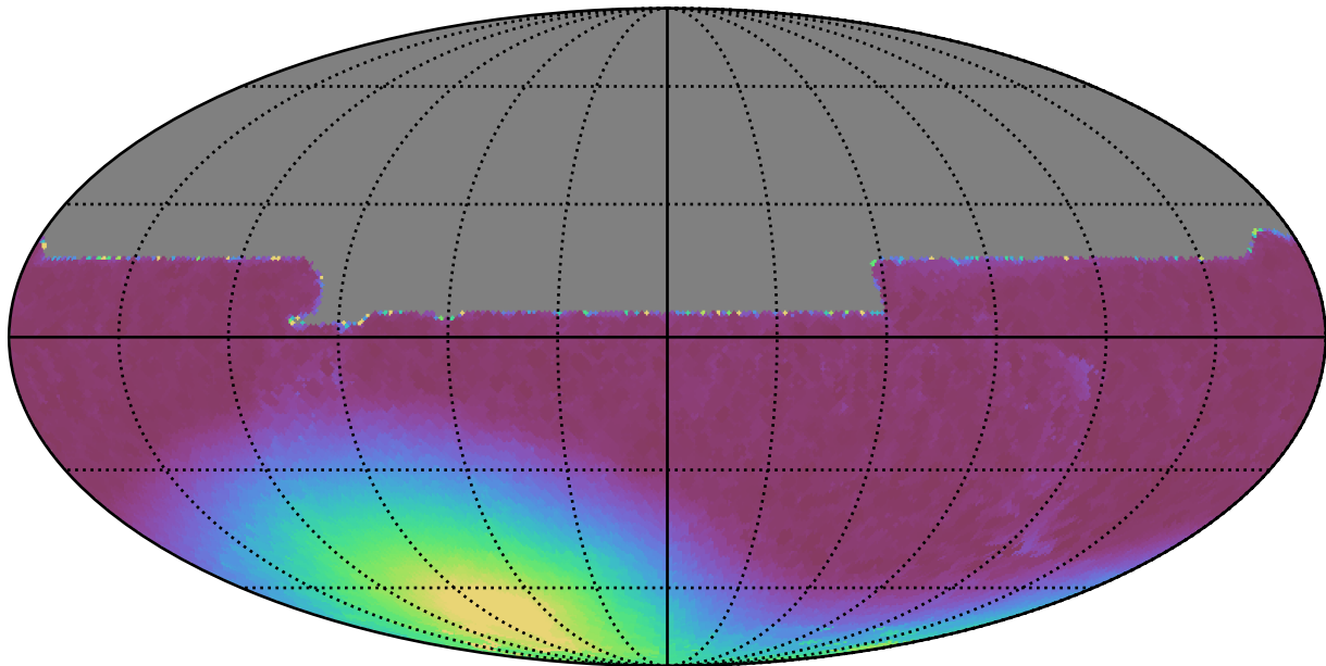
weather_cloudso1v3.4_10yrs All sky y band: Min moonDistance
