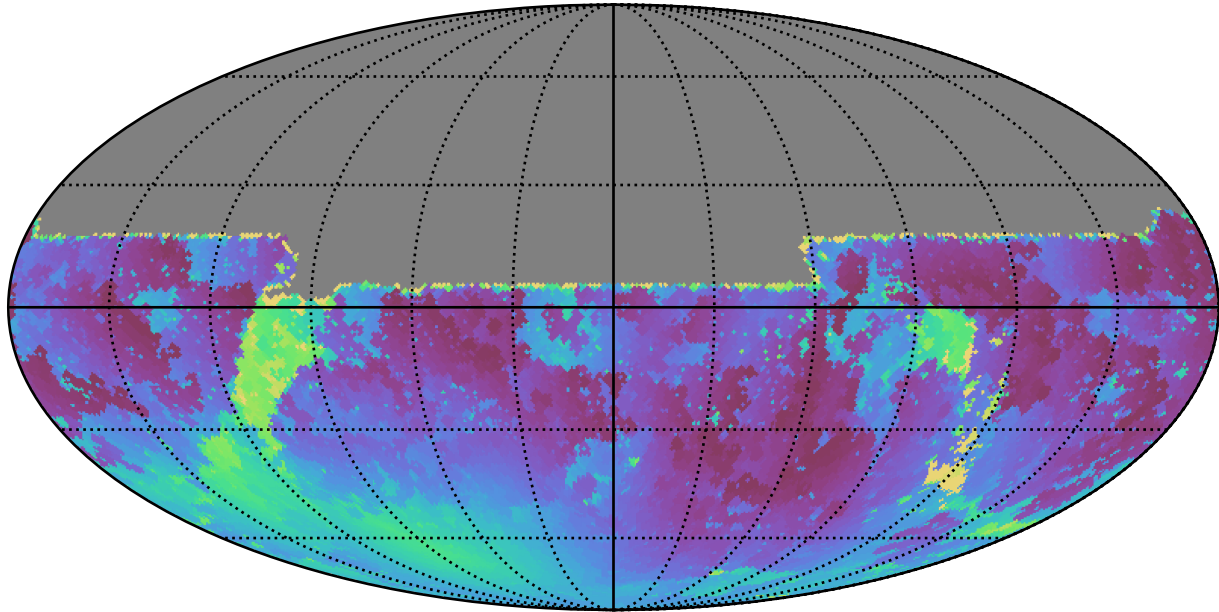
weather_cloudso1v3.4_10yrs All sky u band: Min moonDistance
