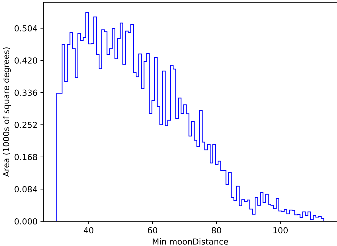
weather_cloudso1v3.4_10yrs All sky u band: Min moonDistance
