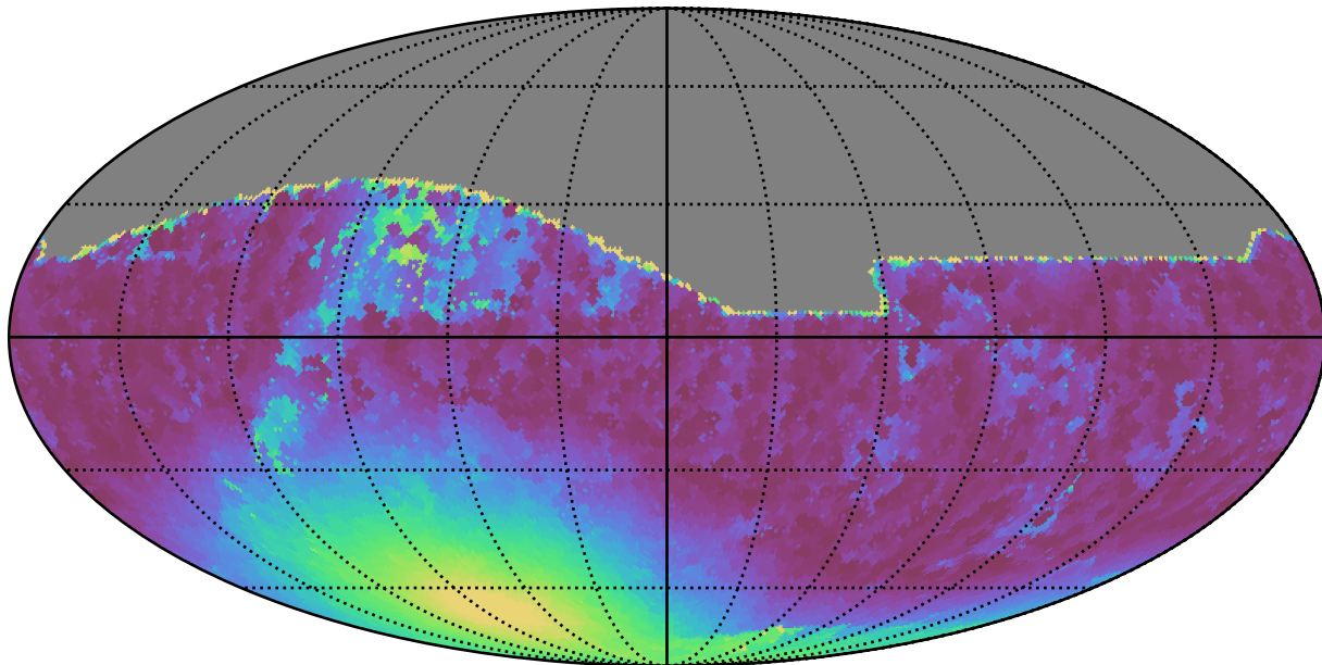
weather_cloudso1v3.4_10yrs All sky r band: Min moonDistance
