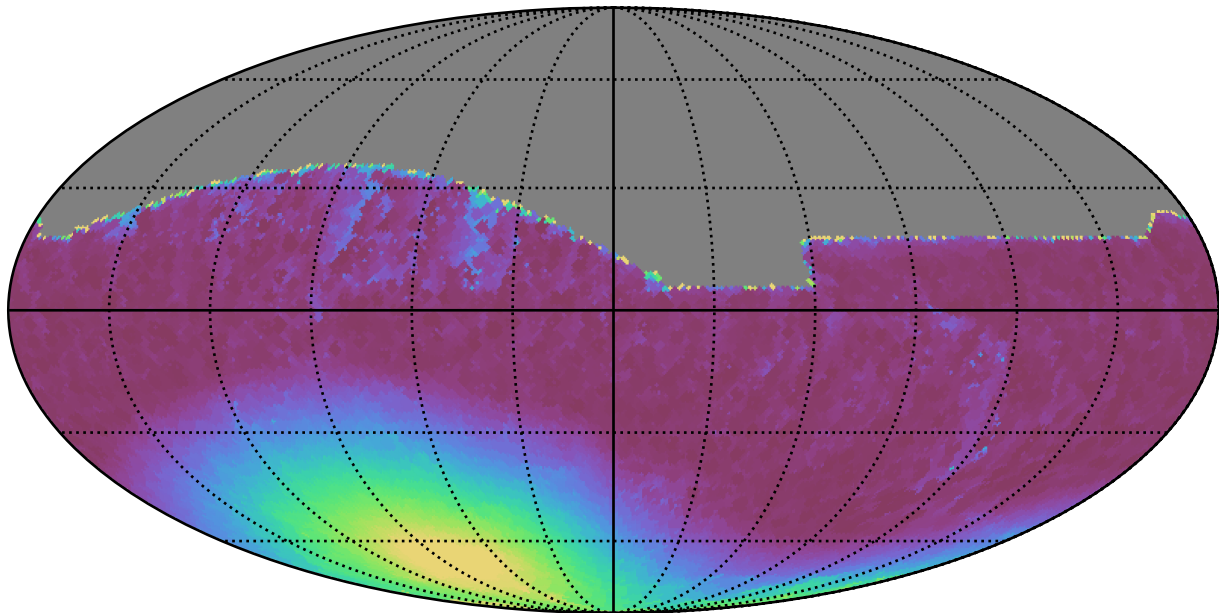
weather_cloudso1v3.4_10yrs All sky i band: Min moonDistance
