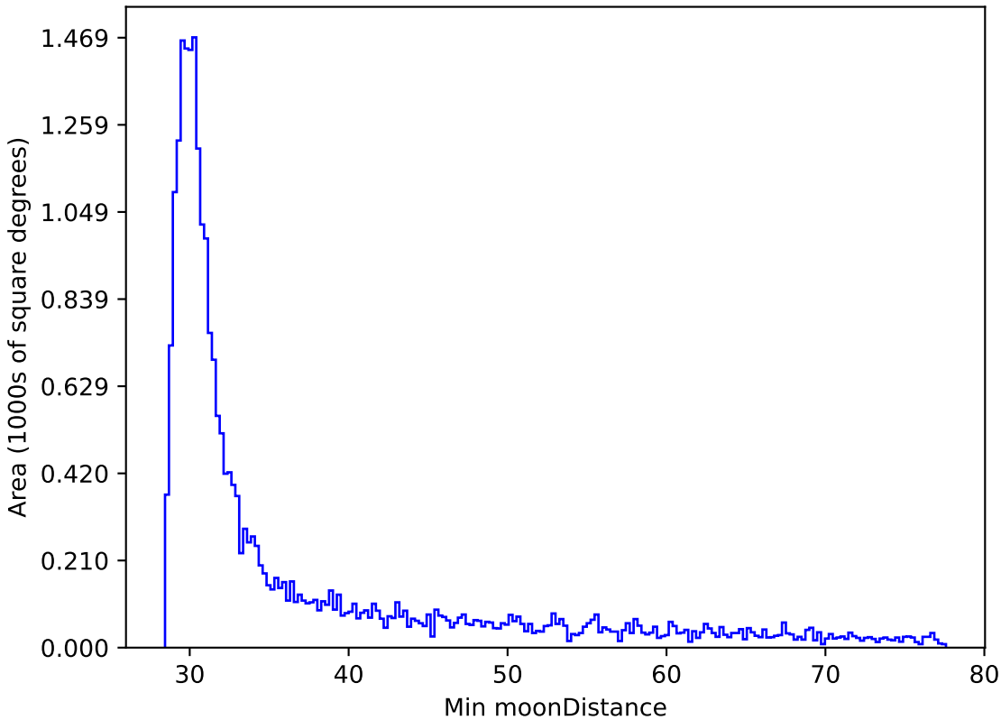
weather_cloudso1v3.4_10yrs All sky i band: Min moonDistance
