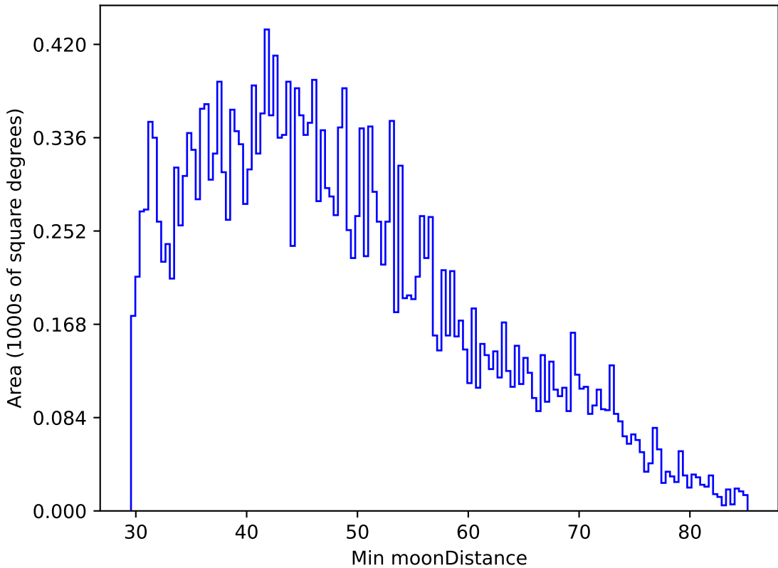
weather_cloudso1v3.4_10yrs All sky g band: Min moonDistance
