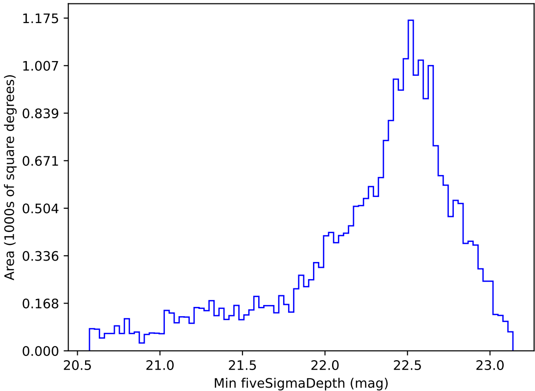
weather_cloudso1v3.4_10yrs Yr 1 z band: Min fiveSigmaDepth
