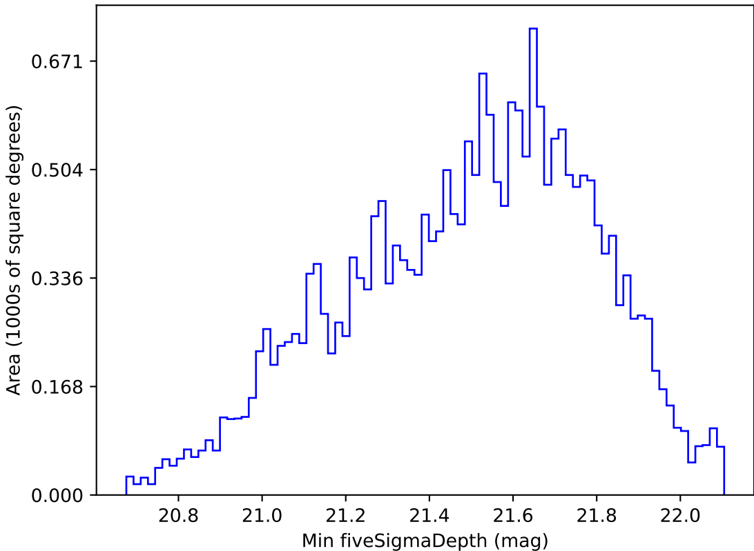
weather_cloudso1v3.4_10yrs Yr 1 y band: Min fiveSigmaDepth
