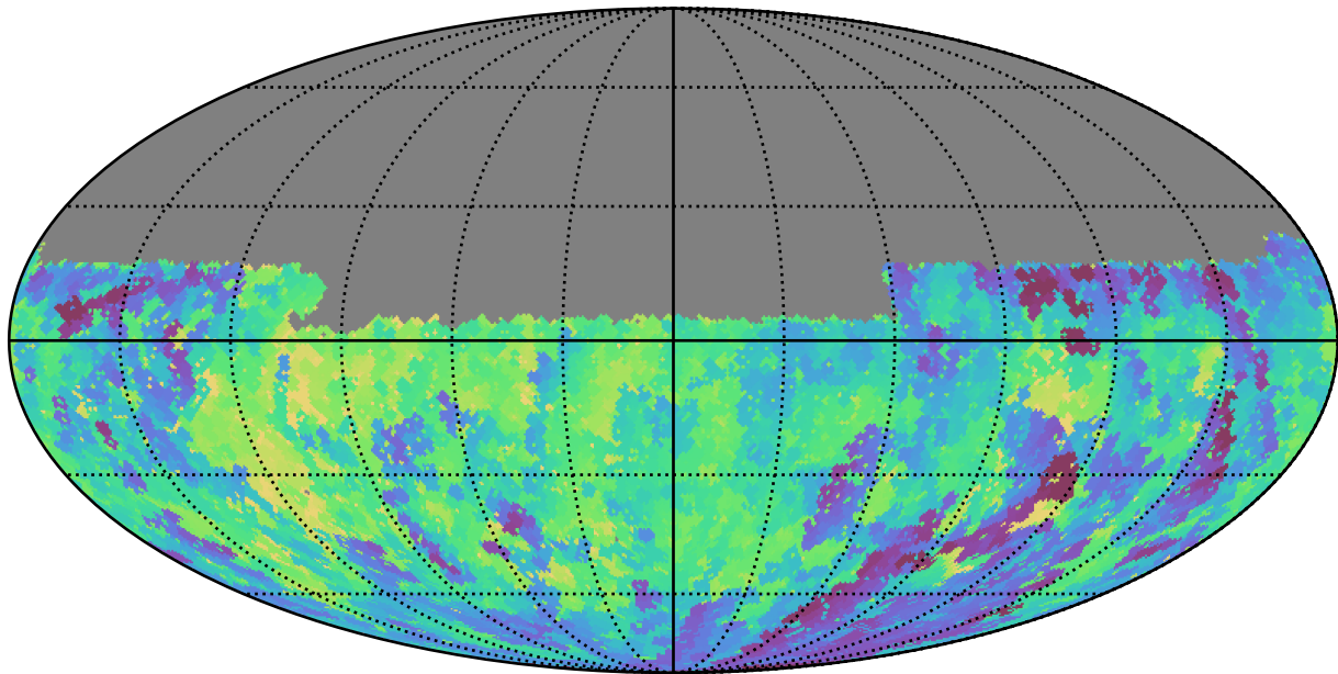
weather_cloudso1v3.4_10yrs Yr 1 u band: Min fiveSigmaDepth
