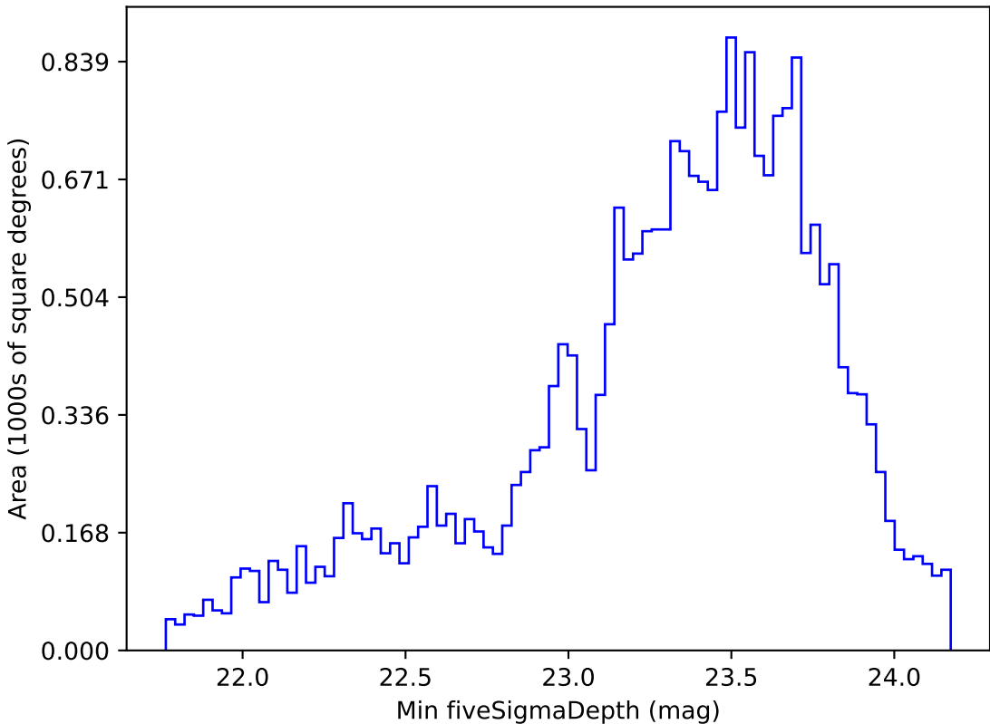
weather_cloudso1v3.4_10yrs Yr 1 r band: Min fiveSigmaDepth
