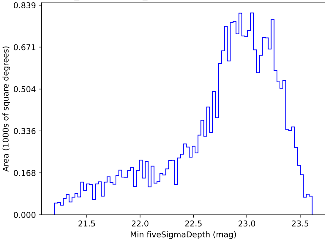
weather_cloudso1v3.4_10yrs Yr 1 i band: Min fiveSigmaDepth
