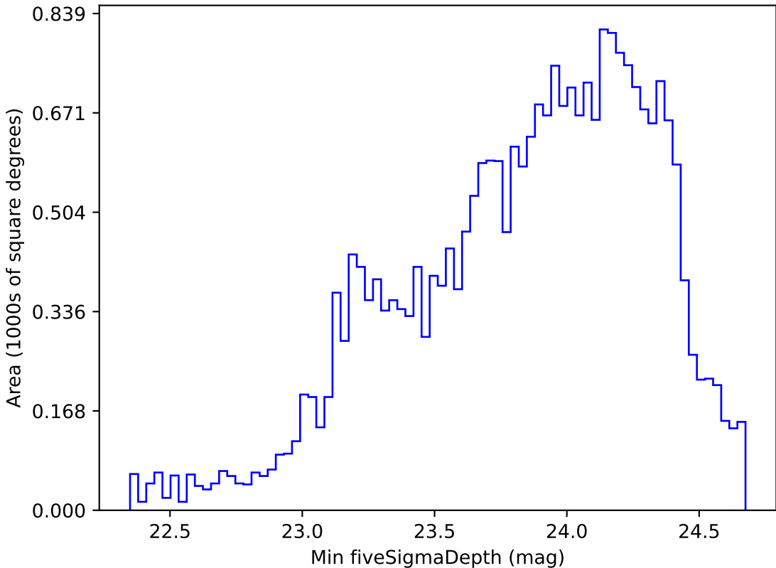
weather_cloudso1v3.4_10yrs Yr 1 g band: Min fiveSigmaDepth
