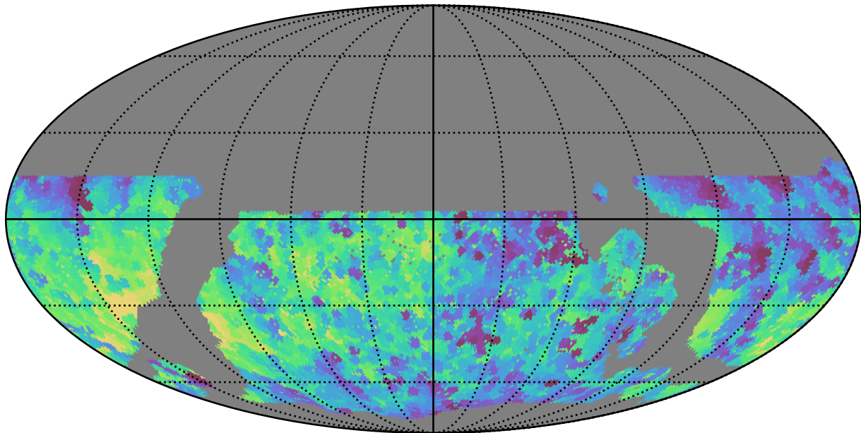
weather_cloudso1v3.4_10yrs WFD y band: Min fiveSigmaDepth
