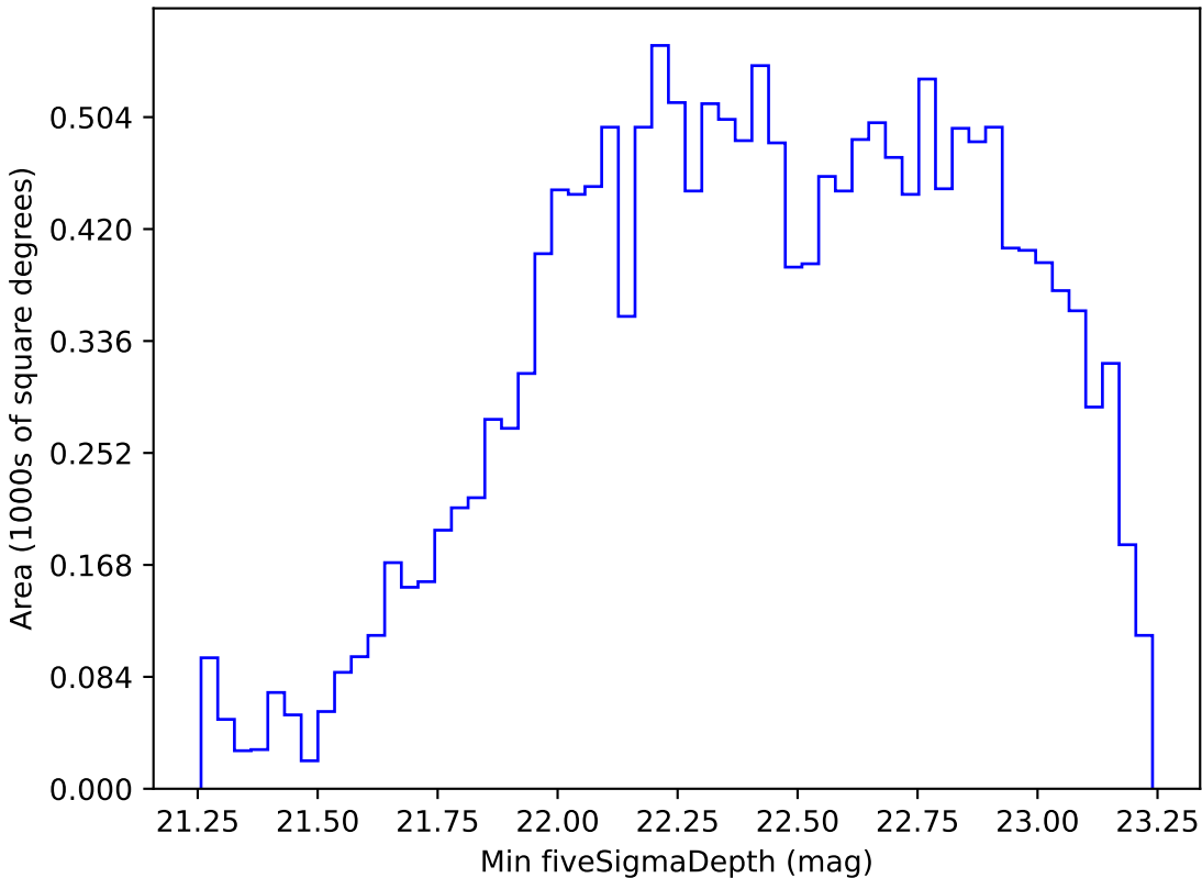
weather_cloudso1v3.4_10yrs WFD r band: Min fiveSigmaDepth
