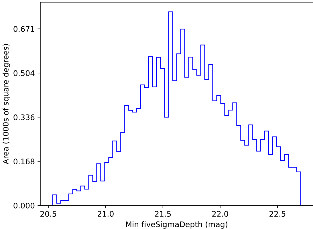
weather_cloudso1v3.4_10yrs WFD i band: Min fiveSigmaDepth
