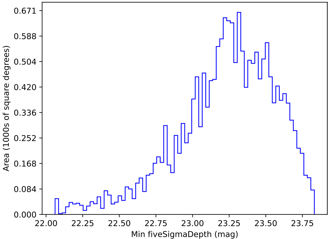
weather_cloudso1v3.4_10yrs WFD g band: Min fiveSigmaDepth
