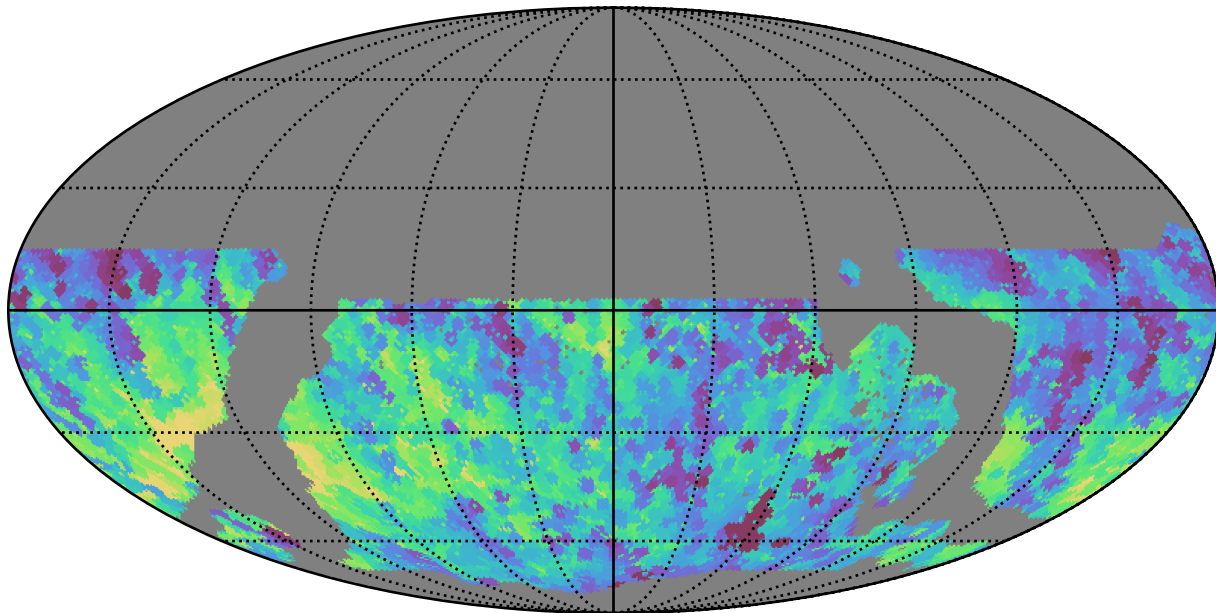
weather_cloudso1v3.4_10yrs WFD all bands: Min fiveSigmaDepth
