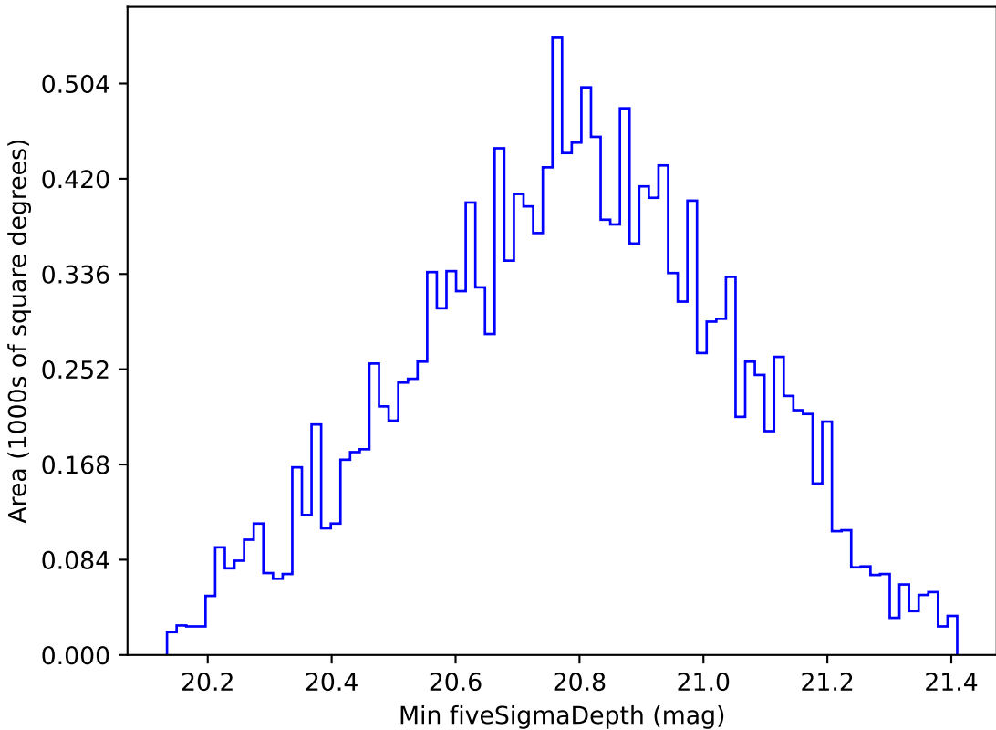
weather_cloudso1v3.4_10yrs WFD all bands: Min fiveSigmaDepth
