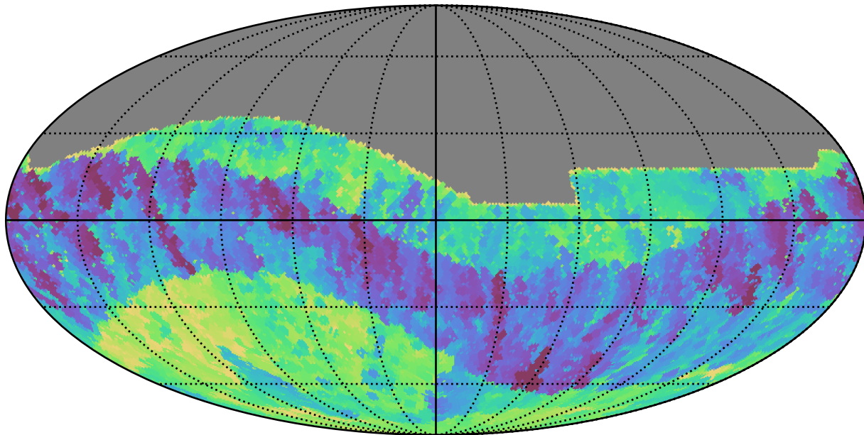
weather_cloudso1v3.4_10yrs All sky z band: Min fiveSigmaDepth
