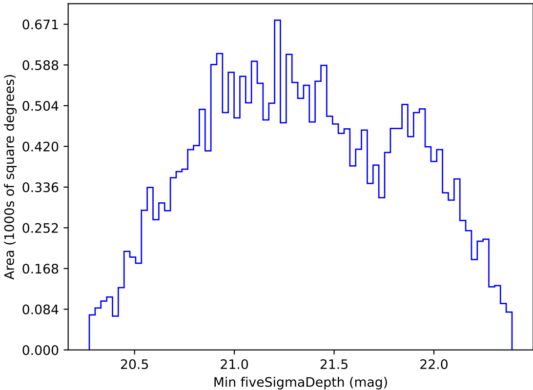
weather_cloudso1v3.4_10yrs All sky z band: Min fiveSigmaDepth
