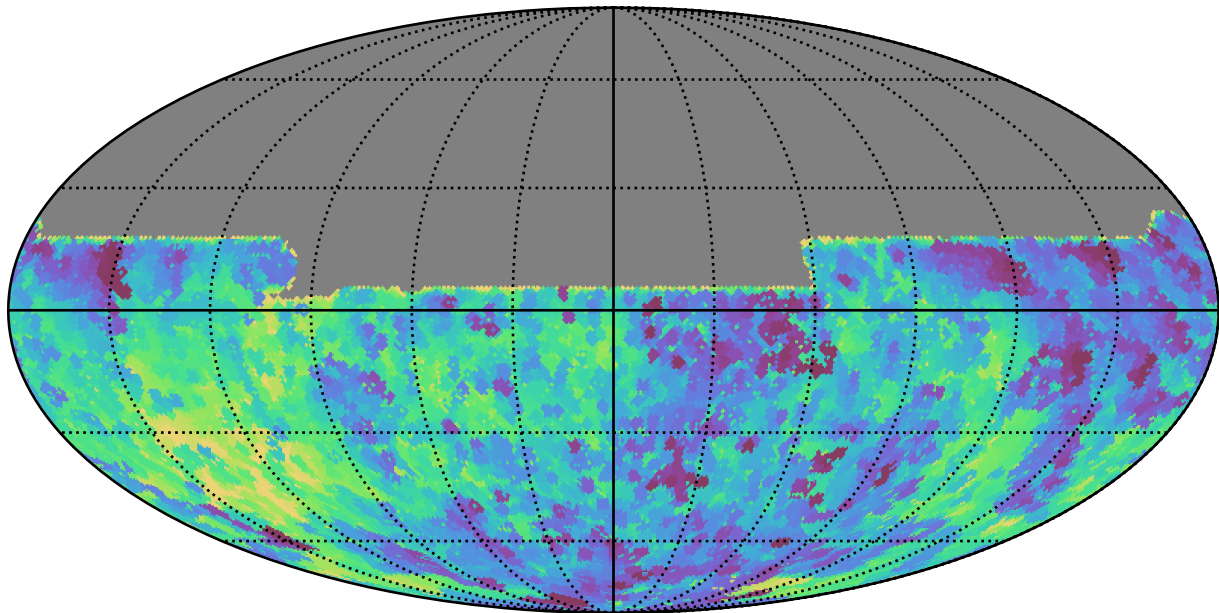
weather_cloudso1v3.4_10yrs All sky y band: Min fiveSigmaDepth
