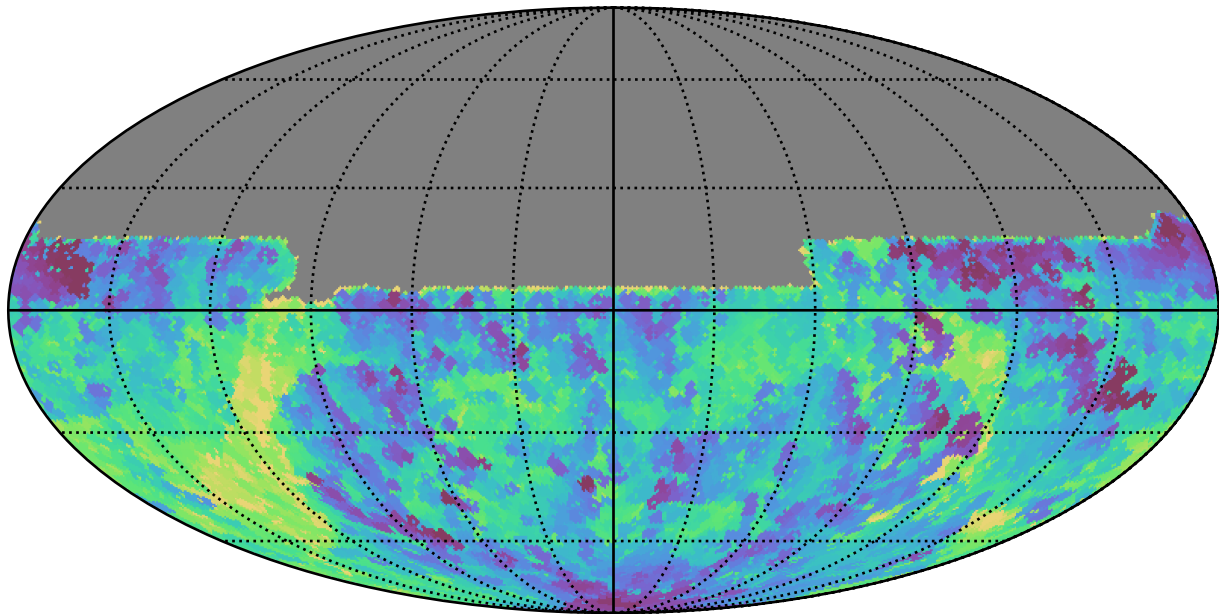
weather_cloudso1v3.4_10yrs All sky u band: Min fiveSigmaDepth
