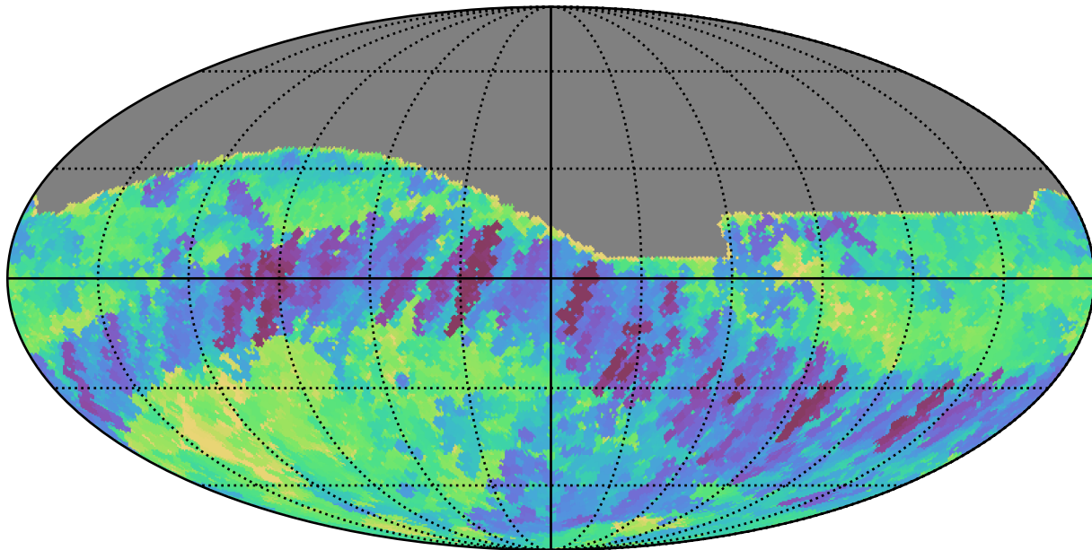
weather_cloudso1v3.4_10yrs All sky r band: Min fiveSigmaDepth
