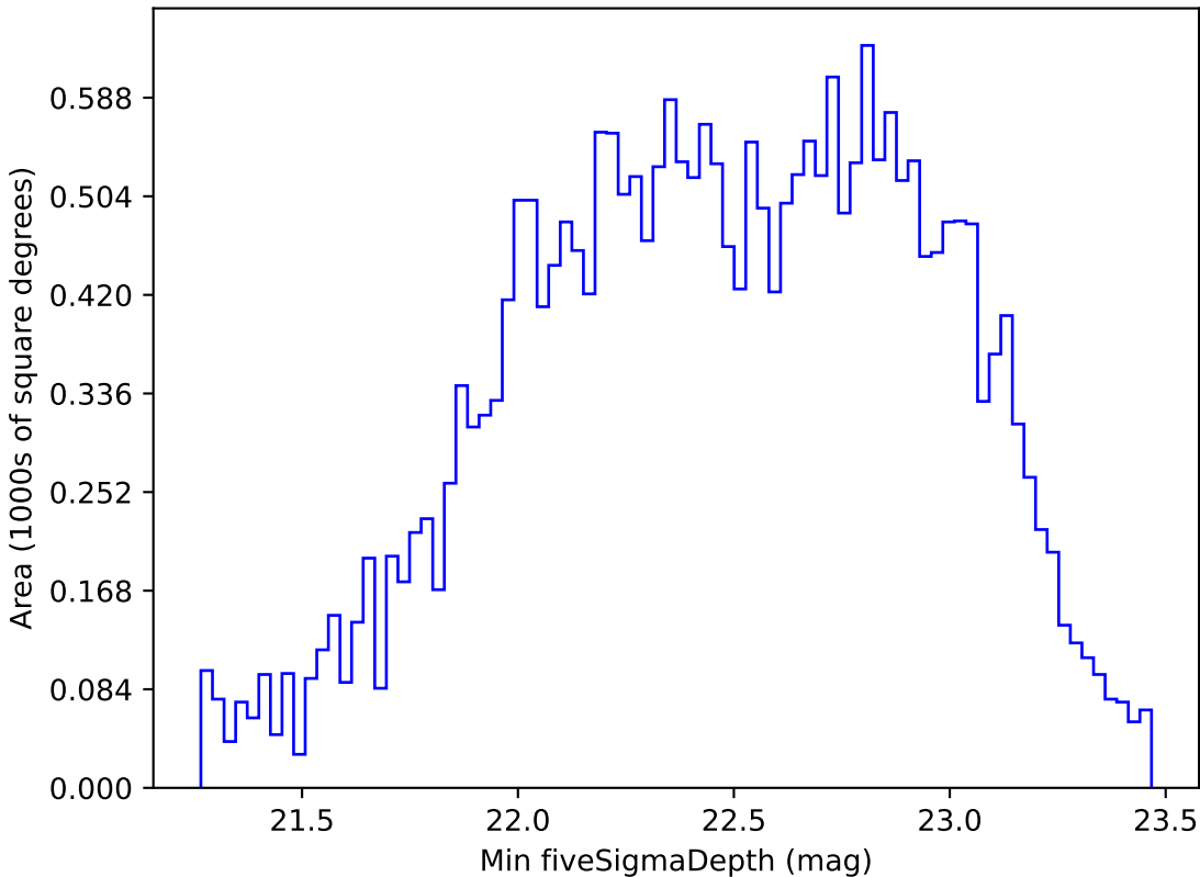
weather_cloudso1v3.4_10yrs All sky r band: Min fiveSigmaDepth
