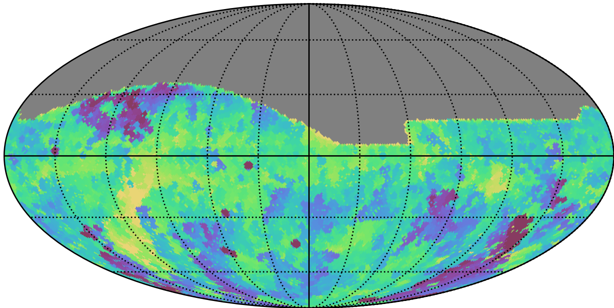
weather_cloudso1v3.4_10yrs All sky g band: Min fiveSigmaDepth
