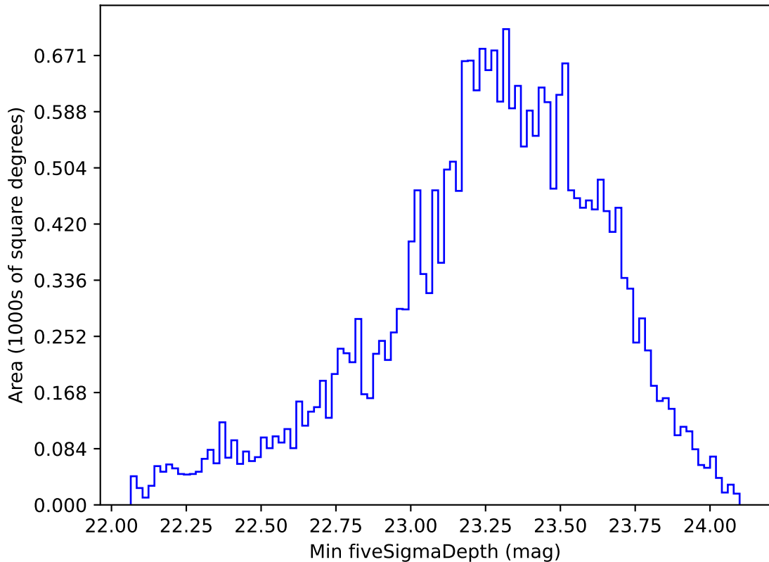
weather_cloudso1v3.4_10yrs All sky g band: Min fiveSigmaDepth
