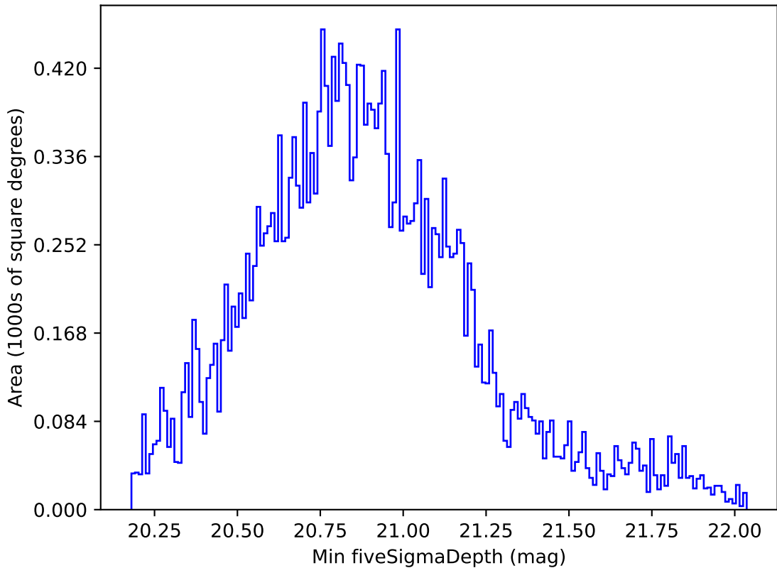
weather_cloudso1v3.4_10yrs All sky all bands: Min fiveSigmaDepth
